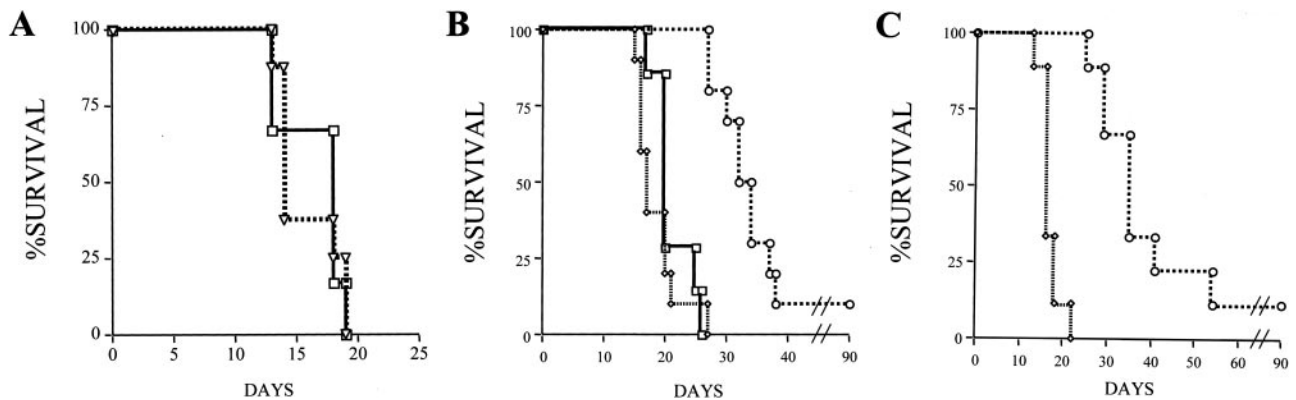
Fig. 4 Kaplan-Meier survival curves of rats bearing established intracranial 9L gliosarcomas tumors treated with 10-mg Paclimer:PEG-1000 (50:50) implants (○). A , systemically administered i.p. Paclimer (▽) did not prolong survival compared with animals receiving no treatment (□). Median survival of i.p. Paclimer-treated animals = 14 days, median survival of control-treated animals = 18 days ( P = 0.0944 ). B , Paclimer (○) implanted intratumorally extended median survival compared with animals receiving no treatment (□). Median survival of Paclimer-treated animals = 33 days, median survival of control-treated animals = 20 days ( P < 0.0001 ). Blank polylactofate:PEG-1000 microspheres (◇). Median survival of Paclimer-treated animals = 33 days, median survival of polylactofate-treated animals = 17 days ( P < 0.0001 ). C , Paclimer (○) extended median survival compared with control groups receiving empty polylactofate:PEG-1000 microspheres (◇). Median survival of Paclimer-treated animals = 35 days, median survival of polylactofate-treated animals = 16 days ( P < 0.001 ). Statistical analysis was performed using the nonparametric Mantel-Cox method with SPSS software.
