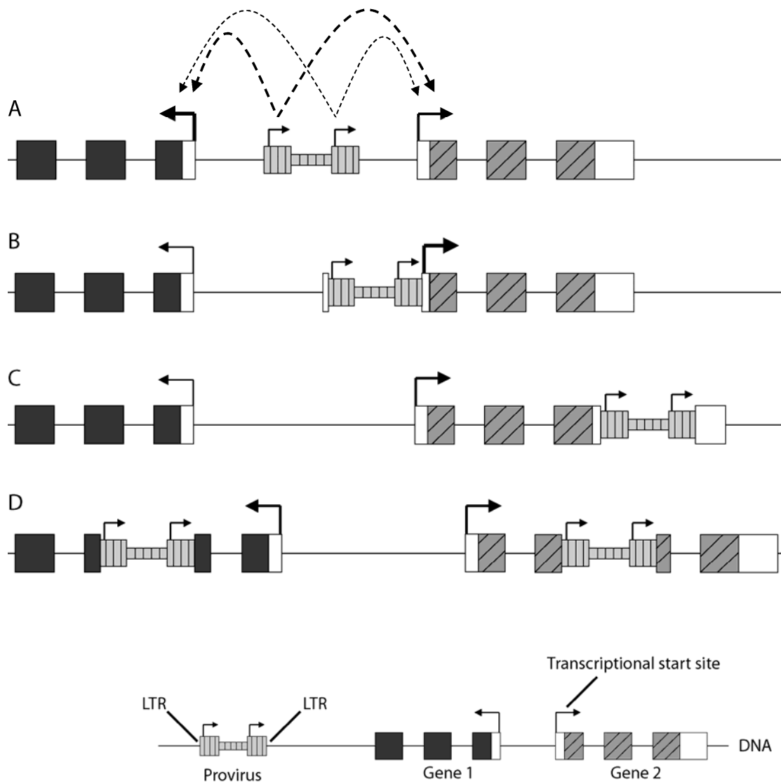
5. Schematic illustration of retroviral insertional mutagenesis. Different modes of proviral activation of Gene 1 and Gene 2 in hypothetical loci in the host cell genome. The unfilled parts of the first exons of the genes represent promoter regions. Integrating proviruses are depicted with two long terminal repeats (LTRs). Arrows denote transcriptional start sites. The thickness of the arrows represents levels of induced expression. A. Viral enhancer activation. The 5' LTR to the right usually provides a stronger enhancer effect than the 3' LTR. B. Viral promoter insertion activation. Either of the LTR promoters can drive transcription of the target gene. When the 5' LTR is used, splicing of viral sequences onto a target gene exon can sometimes be observed. C. Post-transcriptional dysregulation. Activation by enhancement from loss of potential RNA-stabilizing motifs. D. Gene truncation (gene I) or insertional activation (gene II). Different transcripts are likely to occur (not shown). Enhancer functions of viral LTRs are believed to decrease with increasing distance but are most likely active in the cases B-D as well. Adapted from (159)
