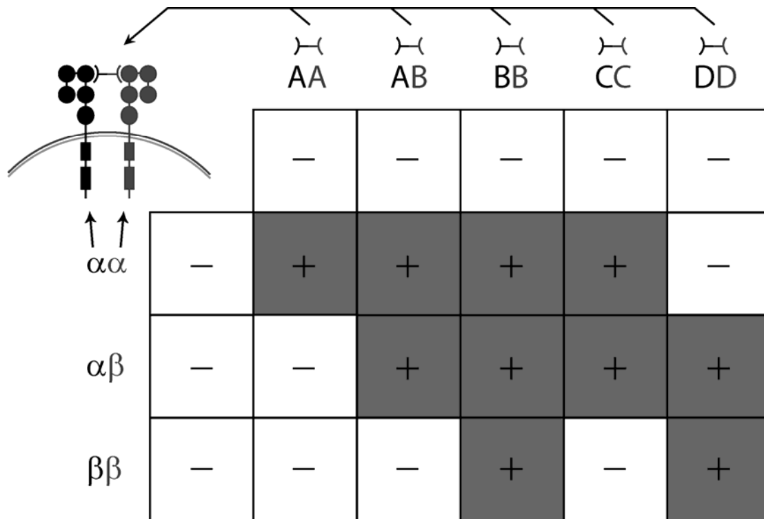
2. The three known PDGF receptor isoforms ( \alpha:\alpha , \alpha:\beta , \beta:\beta ) have different binding capacities for the five known dimeric combinations of the PDGF ligands A-D. The possible pair wise receptor:ligand combinations are shown (boxes). Only the combinations shown in grey with a plus sign will activate an autocrine stimulatory loop.
