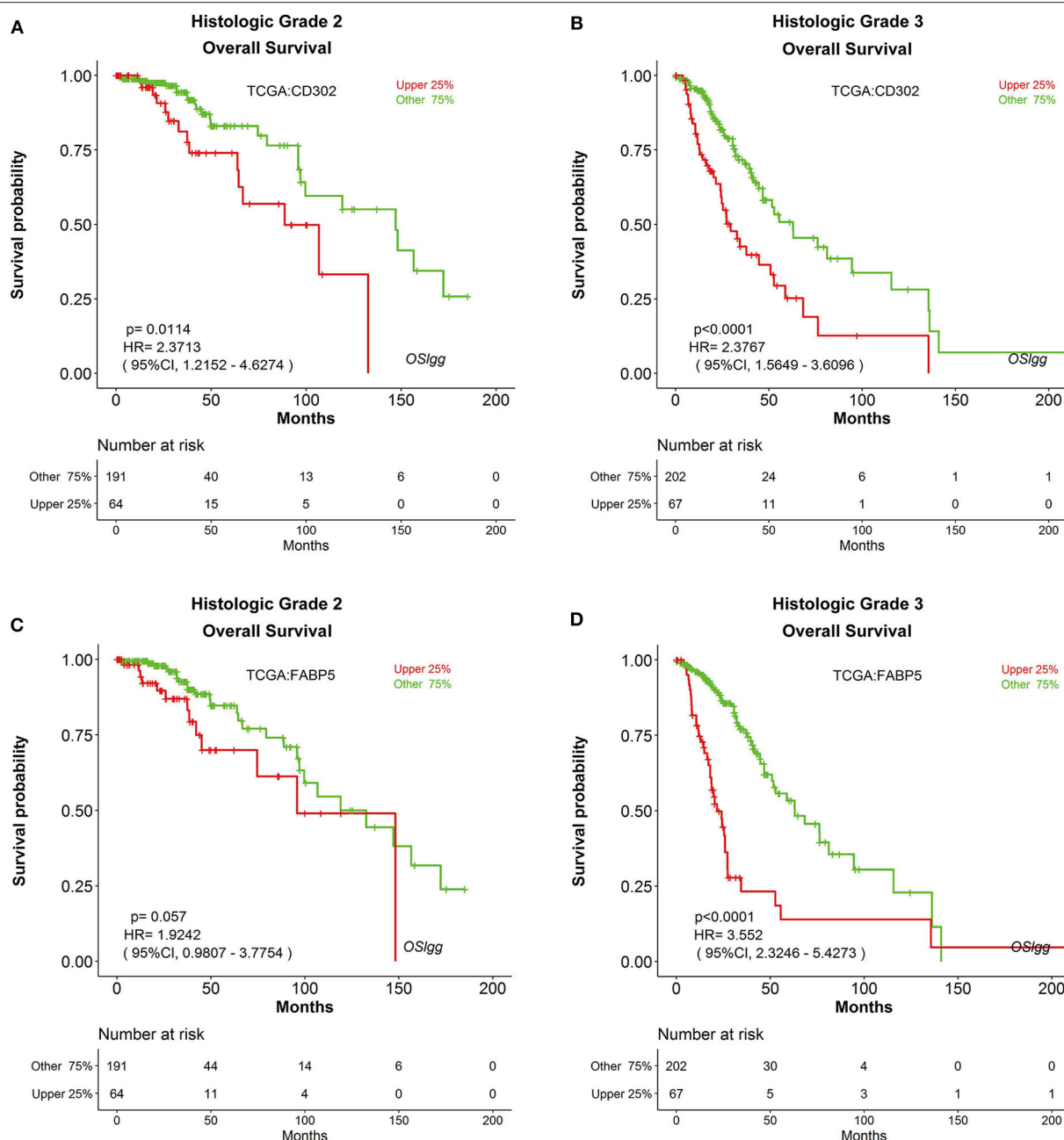
FIGURE 8 | The prognostic abilities of CD302 and FABP5 in terms of histologic grade. Kaplan-Meier plots for CD302 in histologic grade 2 (A) and 3 (B), and for FABP5 in histologic grade 2 (C) and 3 (D), respectively. p -value, confidence interval (95%CI) and number at risk are as shown. The y-axis represents survival rate and the x-axis represents survival time (months).
