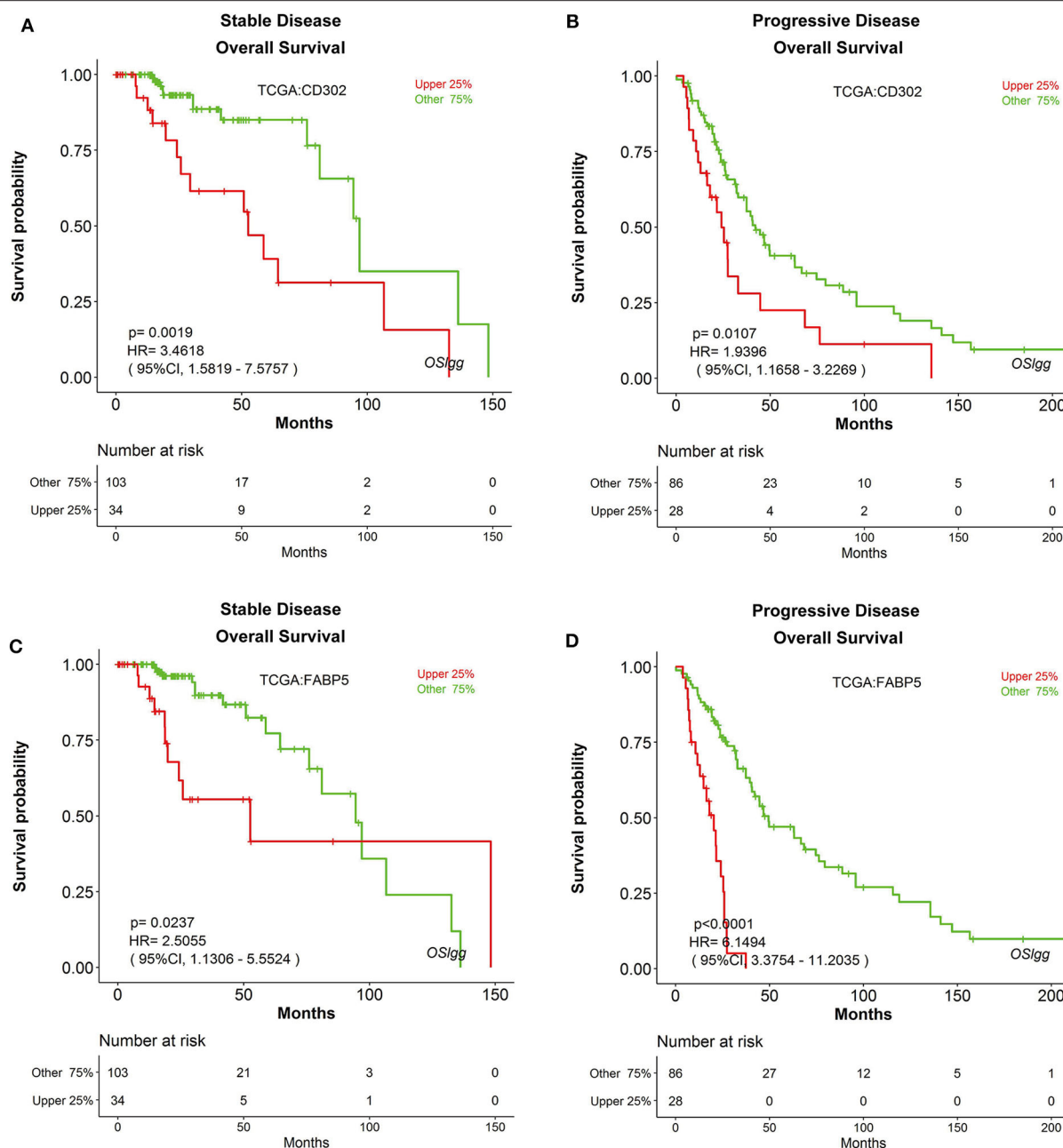
FIGURE 9 | The prognostic abilities of CD302 and FABP5 in terms of primary therapy outcome. Kaplan-Meier plots for CD302 in stable (A) and progressive (B) disease, and for FABP5 in stable (C) and progressive (D) disease, respectively. p -value, confidence interval (95%CI) and number at risk are as shown. The y-axis represents survival rate and the x-axis represents survival time (months).
