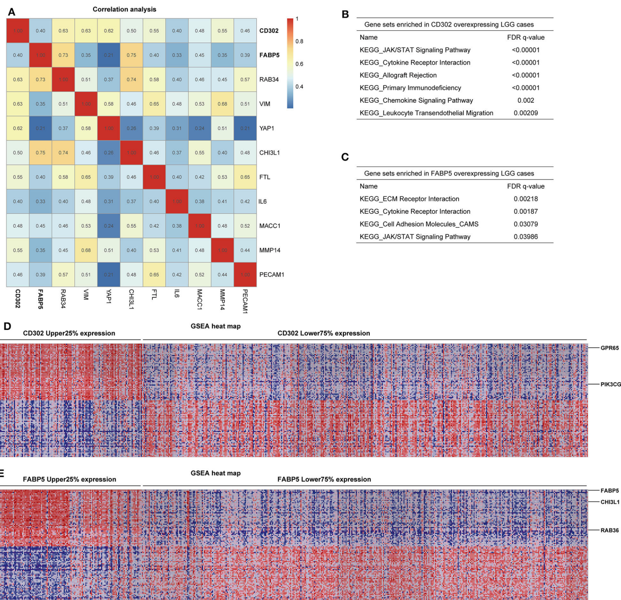
FIGURE 7 | Correlation and GSEA analysis of CD302 and FABP5 . (A) Correlation analysis between CD302 or FABP5 and the previously reported prognostic biomarkers by Spearman's rank correlation test with correlation coefficient marked on the matrix plot. (B–E) GSEA analysis of tumors with high versus low expression of CD302 and FABP5 . LGG patients were split into two subgroups according to CD302 or FABP5 expression, named as CD302 or FABP5 Upper 25% expression and Lower 75% expression. (B,C) Gene sets enriched in CD302 and FABP5 overexpressing LGG cases, respectively. (D,E) GSEA heat maps for differential expression genes enriched in CD302 and FABP5 overexpressing LGG cases, respectively.
