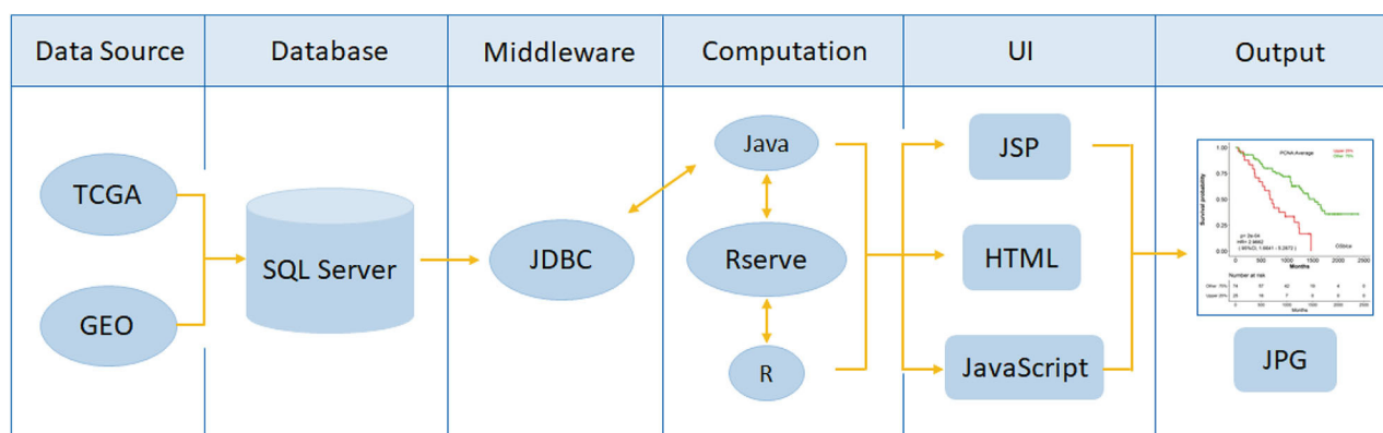
FIGURE 1 | Flowchart of web server OSlgg architecture.
