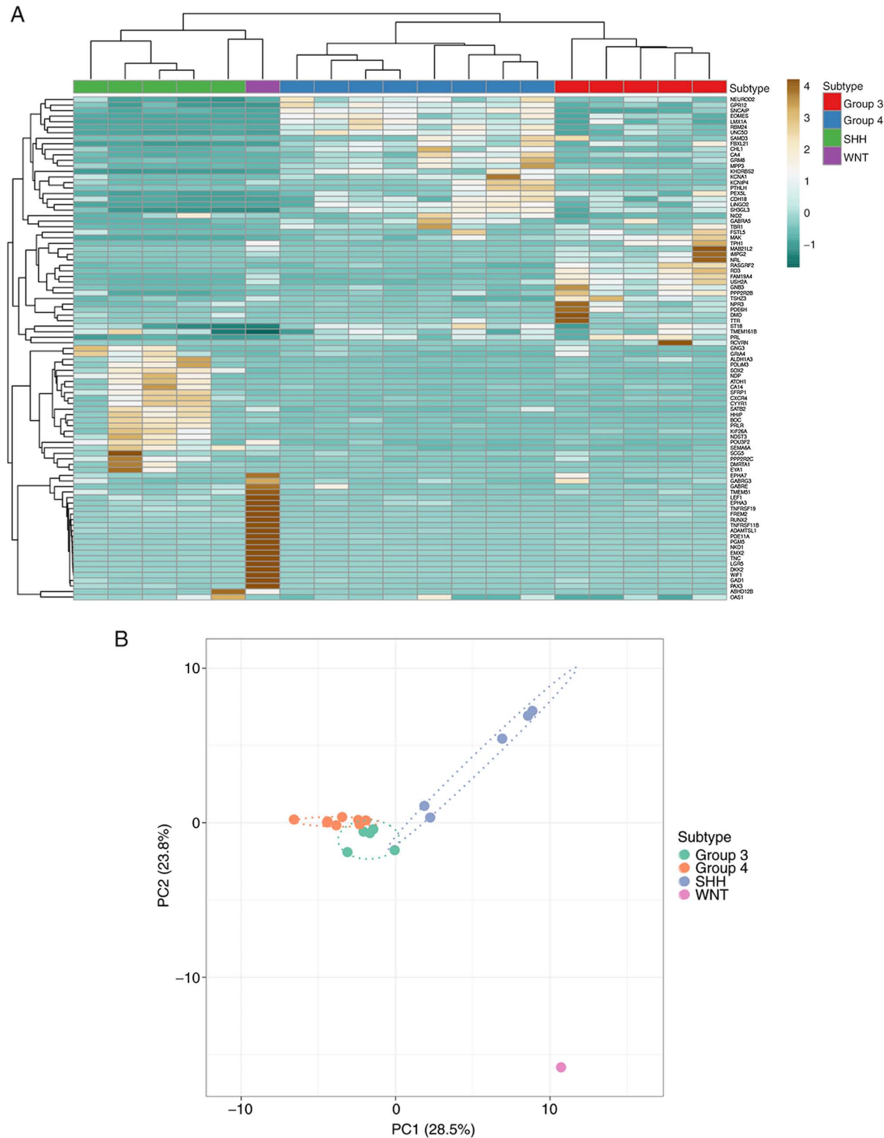
Figure 1. Identification of molecular subgroups. (A) Heatmap of the expression levels of 84 subgroup-specific signature genes. (B) PC analysis demonstrated the degree of separation between the four subgroups. PC, principal component.
