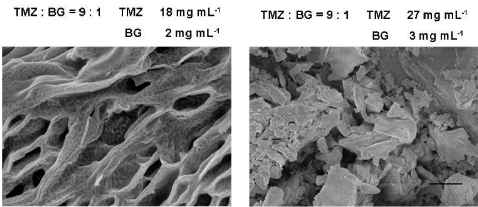
Figure S1. SEM images show a clear 3D porous network of different drug concentrations in the Tm hydrogel. Scale bar = 4 μm.
