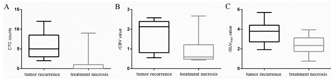
Figure 3. Box-and-whisker plots for CTCs counts, rCBV value and rSUV max value in TR (tumor recurrence) and TN (treatment necrosis) group.
