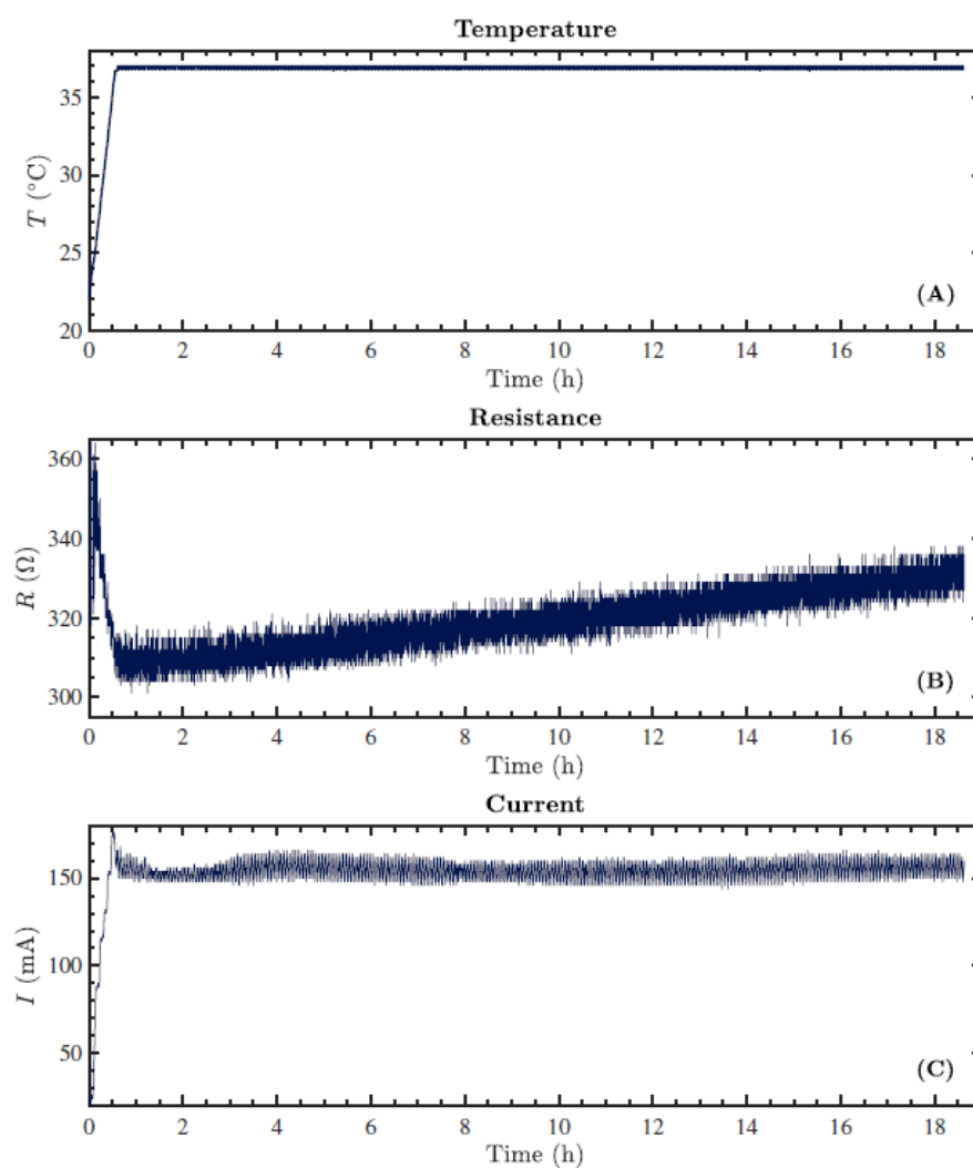
Figure 2. Representative graphs obtained from data logged every 3 s by the inovitro™ live system throughout the exposure of HeLa cells to TTFields with the following parameters: a frequency of 100 kHz, the target medium temperature set to 37 °C, a duty cycle of 1-1, and a duration of ~18 h. The ambient temperature was set to 23 °C. (A) The measured temperature ( T ) as a function of time. (B) The measured resistance ( R ) as a function of time. (C) The measured current ( I ) as a function of time.
