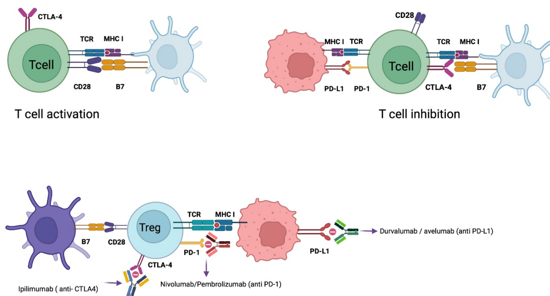
Figure 4. Checkpoint Inhibitors Mechanism of Action. Tumor cells evade the immune system as a defense mechanism. PD-L1 expression on tumor cells binds to PD-1 expressed on T cells, generating anergy of cytotoxic T cells. CTLA-4 expressed on T cells when it binds to B7 increases the expression of T-regs, generating an immunosuppressive response. CTLA-4 has a higher affinity for B7 than CD28 (B7 and CD28 when bound activate cytotoxic T cells). Monoclonal antibodies antagonize CTLA-4, PD-1, and PD-L1 preventing suppression of the immune response by cytotoxic T cells. Abbreviations: CTLA-4, cytotoxic T lymphocyte antigen 4; DC, dendritic cell; MHC, major histocompatibility complex; PD-L1, programmed cell death ligand-1; PD-1, programmed cell death-1; TCR, T-cell receptor; T-regs, regulatory T cells. Created with BioRender.com.
