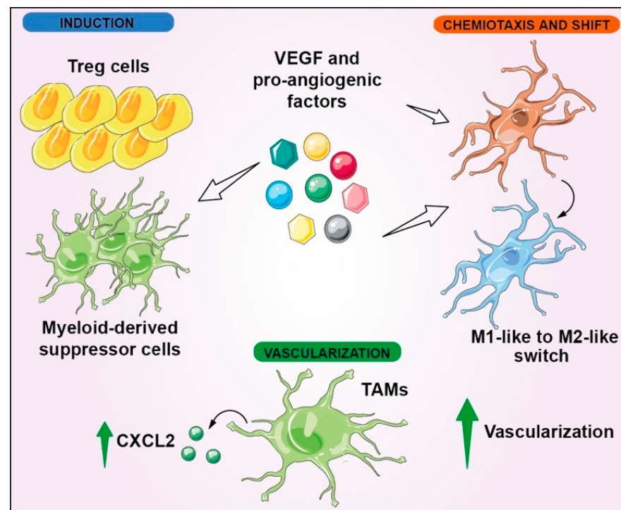
Figure 4. Vascularization and immunomodulation interconnection in GBM. VEGF induces Treg cells and MDSCs; furthermore, it stimulates M1-like to M2-like switch in microglial cells, leading to immune evasion. Moreover, proangiogenic factors, including VEGF, induce chemotaxis of microglial cells. Instead, resident TAMs promote vascularization, upregulating the cell-signaling cytokine CXCL2.
