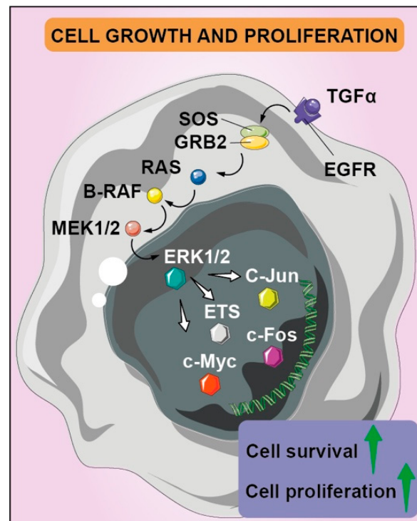
Figure 2. Aberrant regulation of tyrosine kinase receptors determines several signaling pathways' activation, including mitogen-activated protein kinase cascades with pleiotropic effects, such as cell proliferation and survival. EGFR and its mutated version EGFRvIII's overexpression and/or hyper-activation is also fostered by autocrine feedback loop that leads to the transcription of EGFR ligands such as TGFα; the downstream effector Grb2 activates guanine nucleotide exchange factor SOS for GDP/GTP cycling, which promotes formation of active Ras-GTP, binding the other downstream effector targets such as B-Raf. It phosphorylates MEK1 and MEK2 dual-specificity protein kinases, which determine the ERK1 and ERK2 nuclear translocation, where they find several protein targets, such as transcription factors of Ets family, c-MYC and c-JUN. The latter forms a heterodimer with c-FOS, leading to increased cell survival, proliferation, and invasion.
