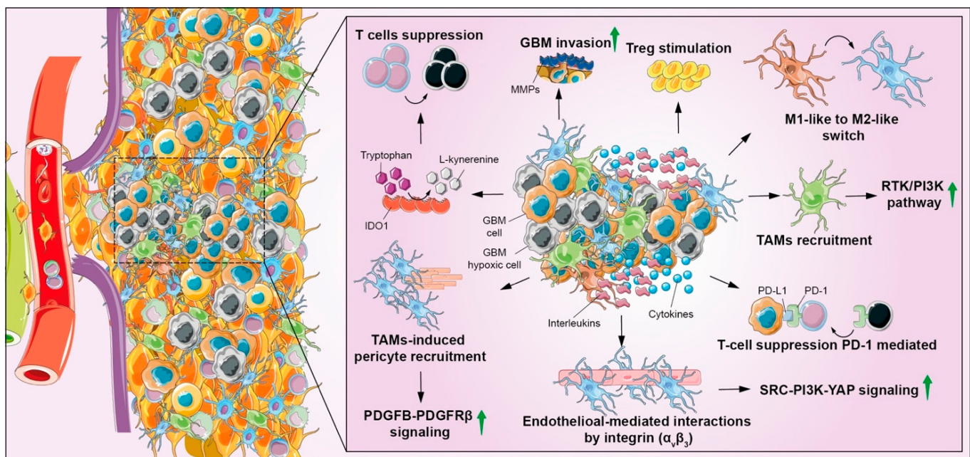
Figure 7. Representation of metabolic reprogramming processes connected GBM invasiveness. The support of GBM invasiveness in hypoxic conditions is not only directly linked to lactate production, but also by indirect effects such as the production of additional signals of molecules such as phosphoglucose isomerase/autocrine-motility factor (PGI/AMF), lipid metabolism and amino-acid reprogramming offer an important contribution to the proinvasion phenotype. Microglia adopts aerobic glycolysis by increasing lactate production and promoting M2 polarization with the concomitant production of cytokines and other factors that can directly suppress effector cells or indirectly via other types of immune cells such as intratumoral DCs and Treg cells, resulting in immunosuppression.
