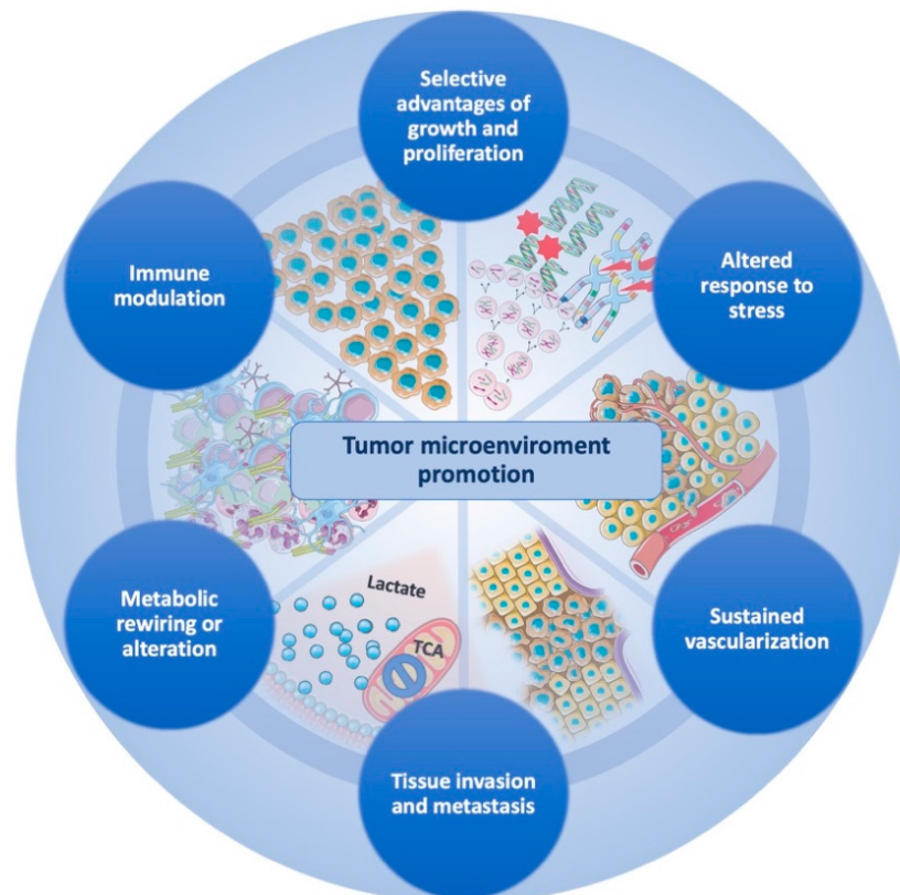
Figure 1. Glioblastoma-tumor microenvironment promotion is ensured by the coexistence of interconnected cancer hallmarks that act with several strategies to achieve tumor maintenance and progression. The circular structure holding the hallmarks emphasizes the cooperation that GBM cells exert to create an ultimate tumor microenvironment that supports survival and progression of cancer cells.
