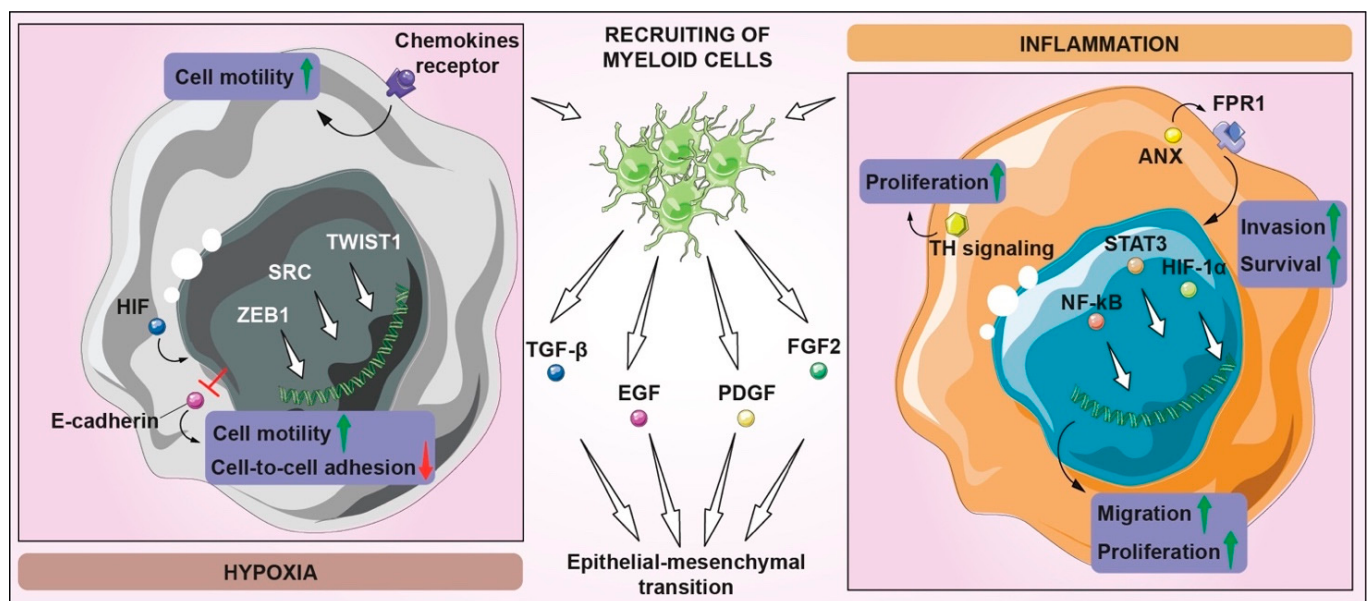
Figure 5. Tissue invasion and metastasis in GBM. Many pathways are involved in the invasion processes of GBM, especially in hypoxic and inflammatory contexts. Hypoxic and inflammatory conditions lead to the recruitment of myeloid cells, which promote TGF- \beta , EGF, PDGF, and FGF2 signaling, triggering the EMT initiation. In hypoxic conditions, HIFs regulate ZEB1, inhibiting E-cadherin expression, which contributes to the loss of cell–cell adhesion and the increase in motility, also supported by the activation of TWIST1, SRC, and chemokine receptors. In the inflammatory context, the upregulation of proinflammatory genes determines an increase in migration and proliferation, while ANX, through the FPR1 activation, induces the heightening of invasion and survival ability by means of STAT3, NF- \kappa B, and HIF-1 \alpha pathways. Moreover, proliferation is also promoted by TH signaling, derived from microglia-GBM crosstalk.
