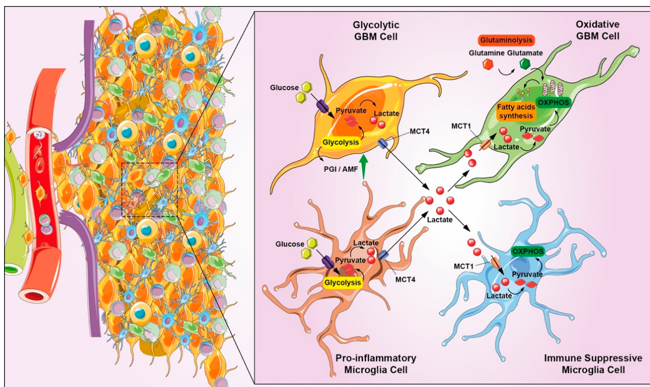
Figure 6. Representation of metabolic reprogramming processes connected GBM invasiveness. The support of GBM invasiveness in hypoxic conditions is not only directly linked to lactate production, but also by indirect effects such as the production of additional signals of molecules such as PGI/AMF, and lipid metabolism and amino-acid reprogramming offers an important contribution to the proinvasion phenotype. Microglia adopts aerobic glycolysis by increasing lactate production and promoting M2 polarization with concomitant production of cytokines and other factors that can directly suppress effector cells, or indirectly via other types of immune cells such as intratumoral DCs and Treg cells, resulting in immunosuppression.
