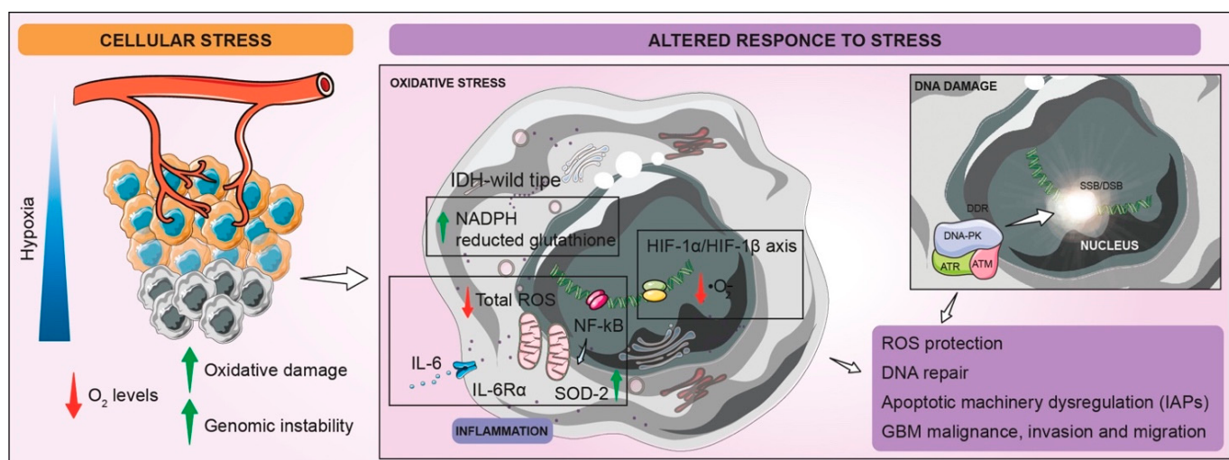
Figure 3. Schematic representation of altered GBM cells responses to stress. The typical condition of hypoxia that characterize GBM TME leads to an increased amount of mitochondrial and intracellular ROS and heightened genome instability. Low levels of O 2 induce stabilization and activation of HIF-1 \alpha /HIF-1 \beta axis, which improves superoxide-anion ( \cdot\text{O}_2^- ) removal. Inflammatory state of hypoxic cells allows total ROS detoxification by IL-6/IL-6R \alpha enhancing and mitochondrial SOD-2 production, guided by NF- \kappa B signaling-pathway activation. Moreover, restored levels of reduced glutathione by cytosolic and mitochondrial NADPH production in IDH wild-type GBM guarantee the protection from oxidative stress. Finally, stress condition also stimulates DDR, involving DNA-PK, ATR, and ATM recruitment, which ameliorates SSB/DSB repair system. All of these processes aim to overcome oxidative stress and DNA instability, ensuring increased GBM malignance, invasion, and migration.
