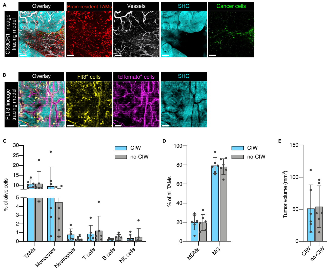
Figure 2. TME characterization of lineage-tracing mouse models
