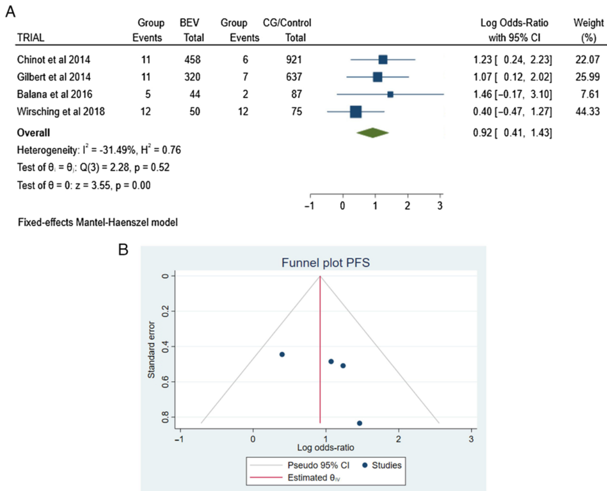
Figure 3. (A) Forest plot PFS. Results demonstrated a statistically significant difference between treatments [OR- 0.92, CI 95% (0.41- 1.43), and P < 0.05 ]. (B) Funnel plot, testing the sensitivity with funnel plot for GCS of admission; there was no statistically significant superiority between groups, with no heterogeneity ( P = 0.52 and I^2 = -31.49\% ). PFS, progression-free survival; OR, Odds Ratio; I^2 shows the percentage of total variation across studies that is due to heterogeneity rather than chance; CI, confidence interval; GCS, Glasgow Coma Scale/Score.
