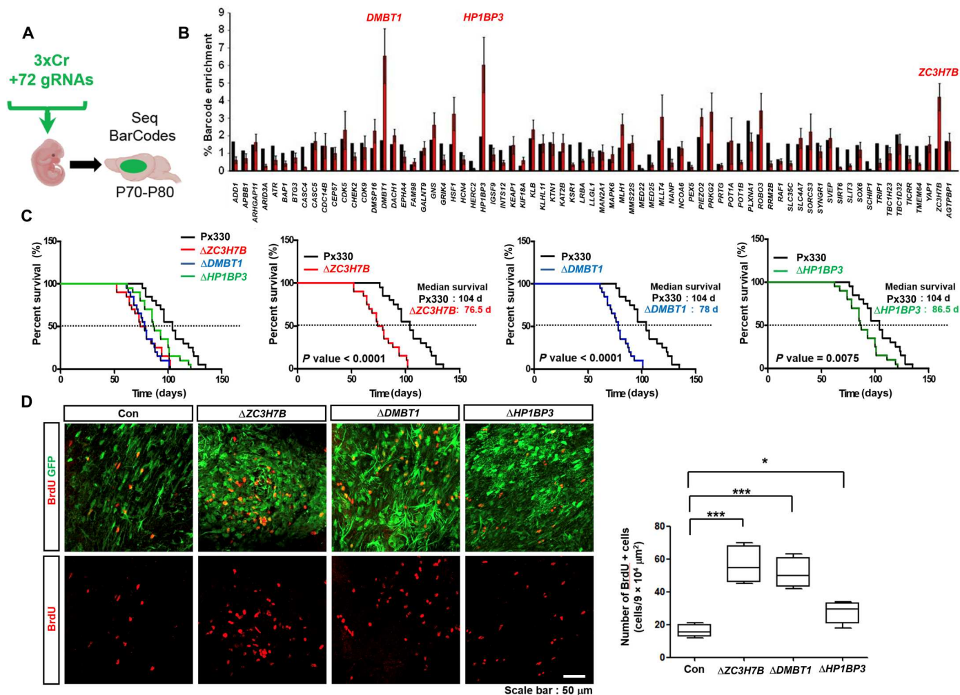
Fig. 5. In vivo functional screening identified regulators of glioma tumorigenesis. (A) Schematic of barcoded screening, where the 3xCr glioma system was combined with 72 barcoded gRNAs and co-electroporated into the embryonic cortex. (B) Next-generation sequencing to determine barcode amplification. The barcode for each gRNA (red) and the input signal (black) are shown ( n = 3 tumors). Data are indicated as the mean and SEM. (C) Kaplan-Meier curves from individual validation studies ( n = 20 , Px330 control, median survival 104 days; n = 20 , \Delta ZC3H7B , median survival 76.5 days; n = 20 , \Delta DMBT1 , median survival 78 days; n = 20 , \Delta HP1BP3 , median survival 86.5 days). (D) BrdU staining of end-stage tumors; quantification for each group is derived from five different tumors. * P < 0.05 , ** P < 0.01 , and *** P < 0.005 . Scale bar, 50 \mu m.
