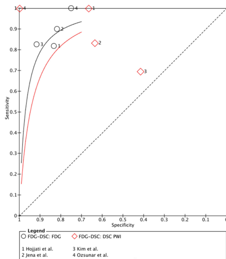
Figure 3. Forest plot and summary receiver operating curves (SROC) of ^{18}\text{F} FDG PET imaging and DSC PW imaging with regard to the differentiation of TP from TRA. ^{18}\text{F} FDG, 2-deoxy-2- ^{18}\text{F} fluoro-D-glucose; DSC PW imaging, dynamic susceptibility contrast perfusion weighted imaging; TP, tumor progression. Forest plot displaying the individual effect sizes from each study for the diagnostic accuracy of ^{18}\text{F} FDG PET imaging and DSC PW imaging with regard to the differentiation of TP from TRA. SROC of ^{18}\text{F} FDG PET imaging (black line) and DSC PW imaging (red line) with regard to the differentiation of TP from TRA shows greater potential for ^{18}\text{F} FDG PET imaging. However, the difference in the diagnostic accuracy of the techniques was not statistically significant [24–26].
