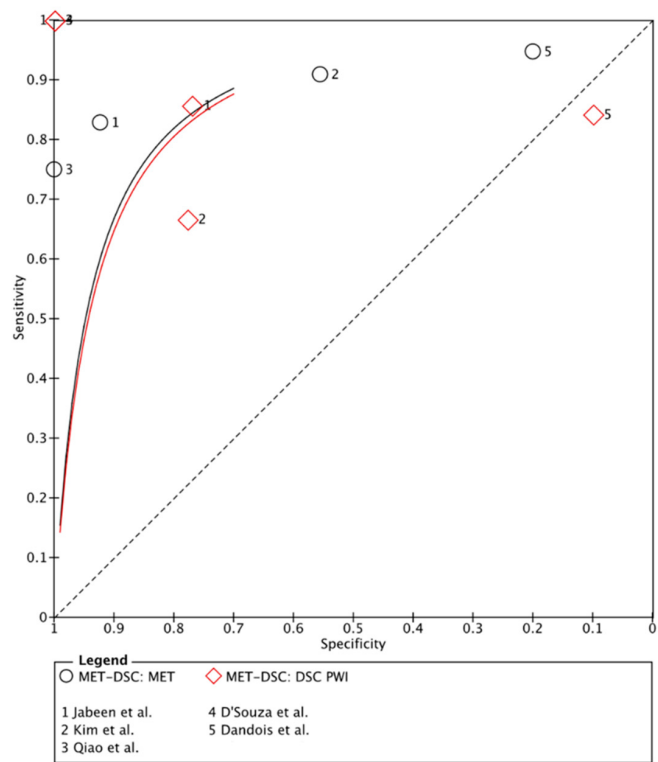
Figure 4. Forest plot and summary receiver operating curves (SROC) of [^{11}\text{C}]\text{MET} PET imaging and DSC PW imaging with regard to the differentiation of TP from TRA. [\text{C}_1\text{-}^{11}\text{C}]\text{MET} , [\text{S-methyl-}^{11}\text{C}]\text{methionine} ; DSC PW imaging, dynamic susceptibility contrast perfusion weighted imaging; TP, tumor progression. Forest plot displaying the individual effect sizes from each study for the diagnostic accuracy of [\text{C}_1\text{-}^{11}\text{C}]\text{MET} PET imaging and DSC PW imaging with regard to the differentiation of TP from TRA. SROC of [\text{C}_1\text{-}^{11}\text{C}]\text{MET} PET imaging (black line) and DSC PW imaging (red line) with regard to the differentiation of TP from TRA shows no superiority of either technique. Additionally, the difference in the diagnostic accuracy of the techniques was not statistically significant [20–23,38].
