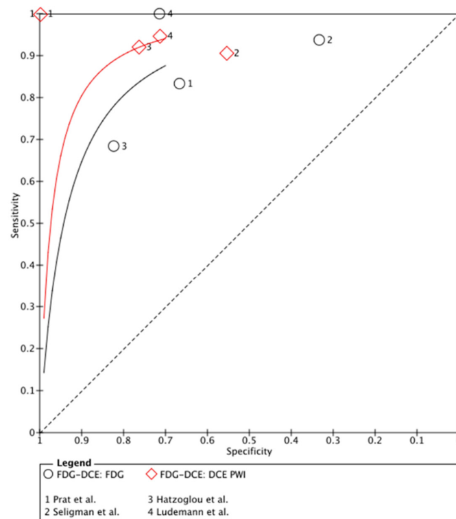
Figure 2. Forest plot and summary receiver operating curves (SROC) of [ ^{18}\text{F} ]FDG PET imaging and DCE PW imaging with regard to the differentiation of TP from TRA. [ ^{18}\text{F} ]FDG, 2-deoxy-2-[ ^{18}\text{F} ]fluoro-D-glucose; DCE PW imaging, dynamic contrast enhancement perfusion weighted imaging; TP, tumor progression. Forest plot displaying the individual effect sizes from each study for the diagnostic accuracy of [ ^{18}\text{F} ]FDG PET imaging and DCE PW imaging with regard to the differentiation of TP from TRA. SROC of [ ^{18}\text{F} ]FDG PET imaging (black line) and DCE PW imaging (red line) with regard to the differentiation of TP from TRA shows greater potential for DCE PW imaging. However, the difference in the diagnostic accuracy of the techniques was not statistically significant [27–30].
