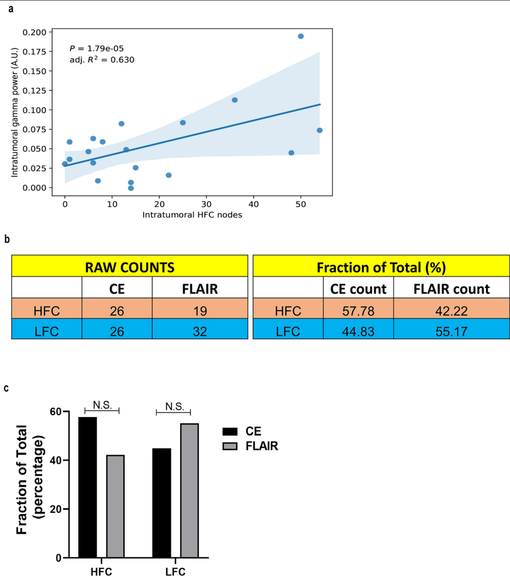
Extended Data Fig. 4 | Gamma power and tumour-intrinsic connectivity imaging correlations. a , Linear regression statistics illustrating that gamma power (a measure of neuronal activity) correlates with number of intratumoural high functional connectivity voxels in glioblastoma (n = 18 patients; P = 0.00002 ). Shaded area represents the 95% confidence interval predicted by the linear regression model. b , Sampling of functionally connected intratumoural regions using MEG was performed exclusively in participants with dominant hemisphere glioblastoma at the point of initial diagnosis. Site-directed tissue biopsies from HFC and LFC regions were taken as determined by MRI. Table illustrates site-
