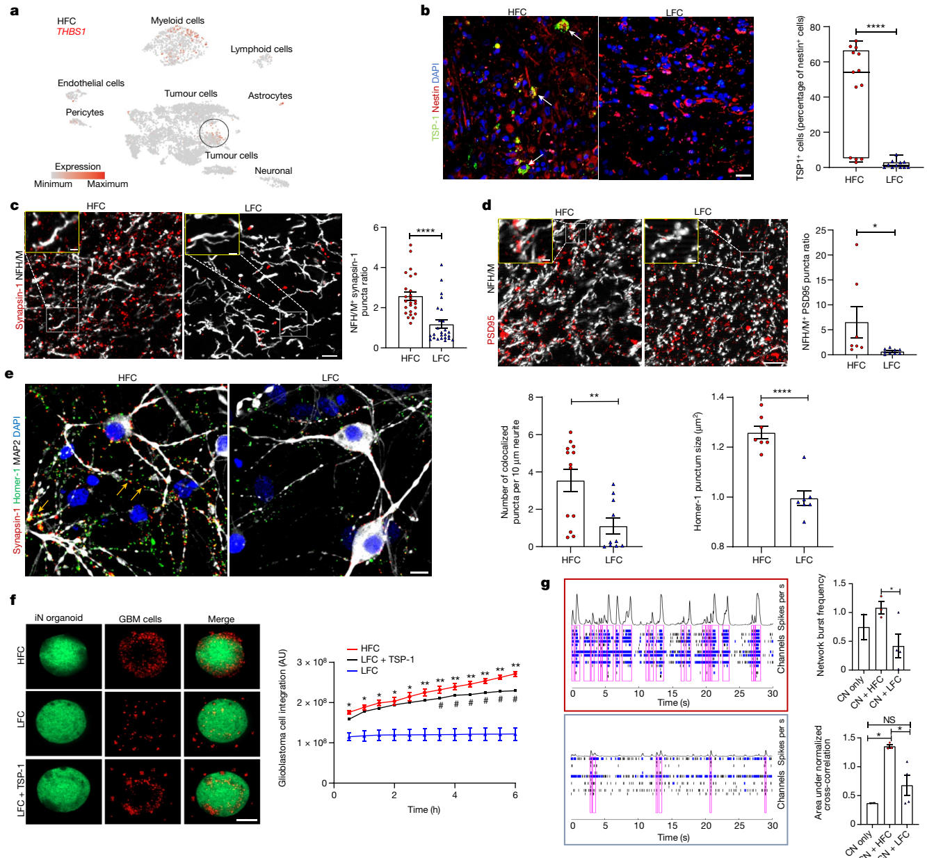
Fig. 2 | Tumour-infiltrated circuits exhibit areas of synaptic remodelling characterized by glioma cells expressing synaptogenic factors. a , Single-cell RNA-seq feature plot analysis of THBS1 in HFC ( n = 6,666 cells, 3 participants) tissues; within HFC samples, THBS1 is primarily in glioblastoma cells (circled). b , TSP-1 immunofluorescence analysis of nestin-positive tumour cells in HFC and LFC tissues. n = 13 (HFC) and n = 11 (LFC) sections, 3 per group. P = 0.000073 . Scale bar, 50 \mu\text{m} . The box plot shows the median (centre line), interquartile range (box limits) and minimum and maximum values (whiskers). c , The synapsin-1 puncta count in HFC and LFC glioblastoma tissue samples. n = 25 regions, 4 per group. P = 0.000014 . Red, synapsin-1 (presynaptic puncta); white, neurofilament heavy and medium (neurons). Scale bar, 10 \mu\text{m} . Inset: magnified view of synapsin-1 puncta on neurons. Scale bar, 3 \mu\text{m} . d , PSD95 puncta count. n = 7 (HFC) and n = 9 (LFC) sections, 3 per group. P = 0.04 . Red, PSD95 (postsynaptic puncta); white, neurofilament heavy and medium chains (NFH/M) (neurons). Scale bar, 10 \mu\text{m} . Inset: magnified view of PSD95 puncta on neurons. Scale bar, 3 \mu\text{m} . e , Representative confocal images showing synaptic punctum colocalization (yellow arrows). Red, synapsin-1; green, homer-1 (postsynaptic puncta); white, MAP2 (neurons); blue, 4',6'-diamidino-2-phenylindole dihydrochloride (DAPI). Scale bar, 10 \mu\text{m} . Quantification of the number of
