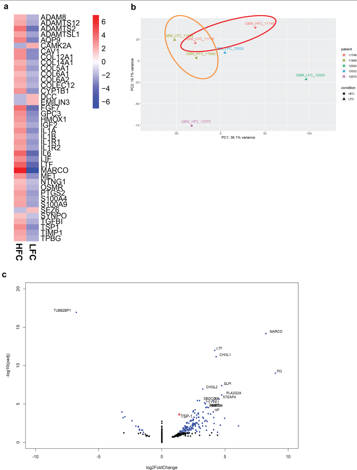
Extended Data Fig. 5 | Neurogenic gene expression in glioblastoma. a, Bulk RNA transcriptomic profile of HFC tissues showed a neurogenic signature including elevated (7-fold) expression of thrombospondin-1 ( TSP-1 ) ( n = 3 -4 per group). b, Unsupervised principal component (PCA) analysis of bulk RNA sequencing data obtained from glioblastoma primary patient HFC ( n = 3 ) and LFC ( n = 4 ) samples. c, Volcano plots of IDH-WT glioblastoma samples revealed
