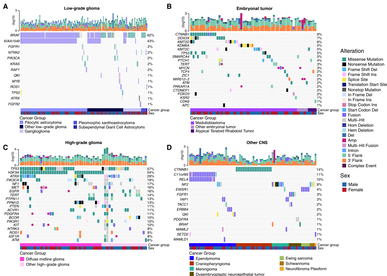
Figure 2. Mutational landscape of PBTA tumors
