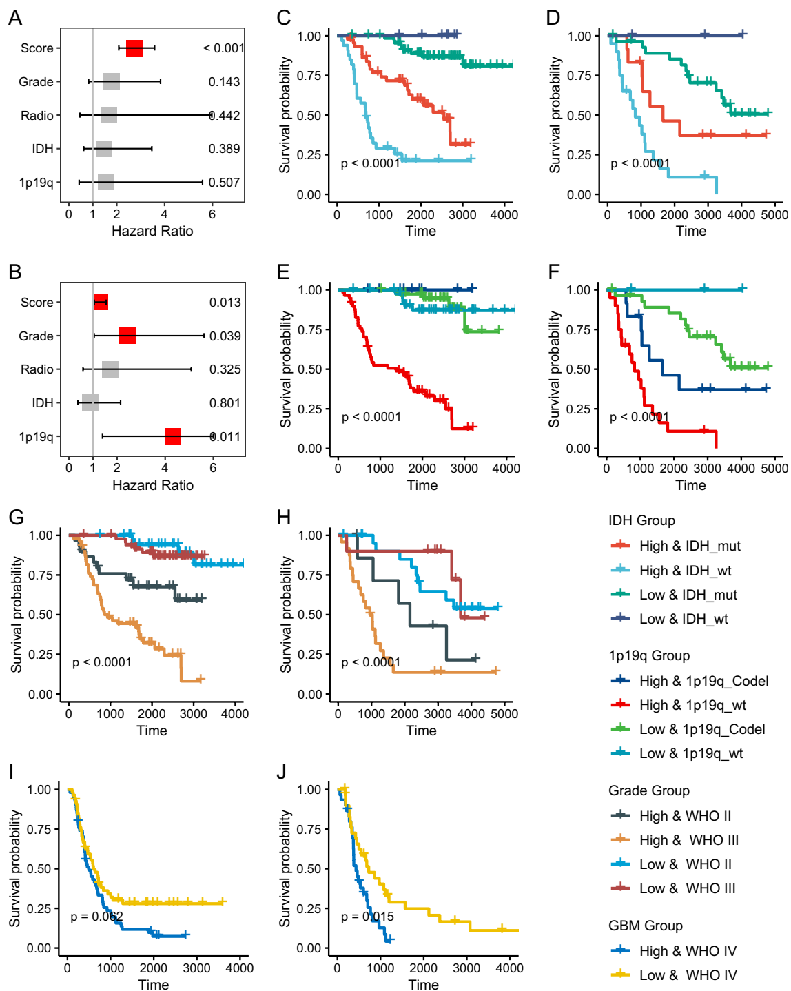
Fig. 3 The prognostic power of risk scores was independent of clinicopathological factors. A Multivariate Cox analysis of risk scores with multiple clinical factors in the training set. B Multivariate Cox analysis of risk scores with multiple clinical factors in the validation set. C Effect of IDH status combined with risk score on survival in the training set. D Effect of IDH status combined with risk score on survival in the validation set. E Effect of chr1p19q co-deletion status combined with risk score on survival in the training set. F Effect of chr1p19q co-deletion status combined with risk score on survival in the validation set. G Effect of WHO grade combined with risk score on survival in the training set. H Effect of WHO grade combined with risk score on survival in the validation set. I Differences in survival curves between high and low risk scores in GBM in CGGA1 datasets. J Differences in survival curves between high and low risk scores in GBM in CGGA2 datasets
