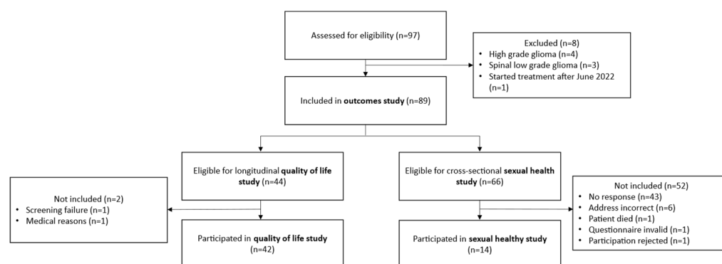
Figure 1. CONSORT diagram.
