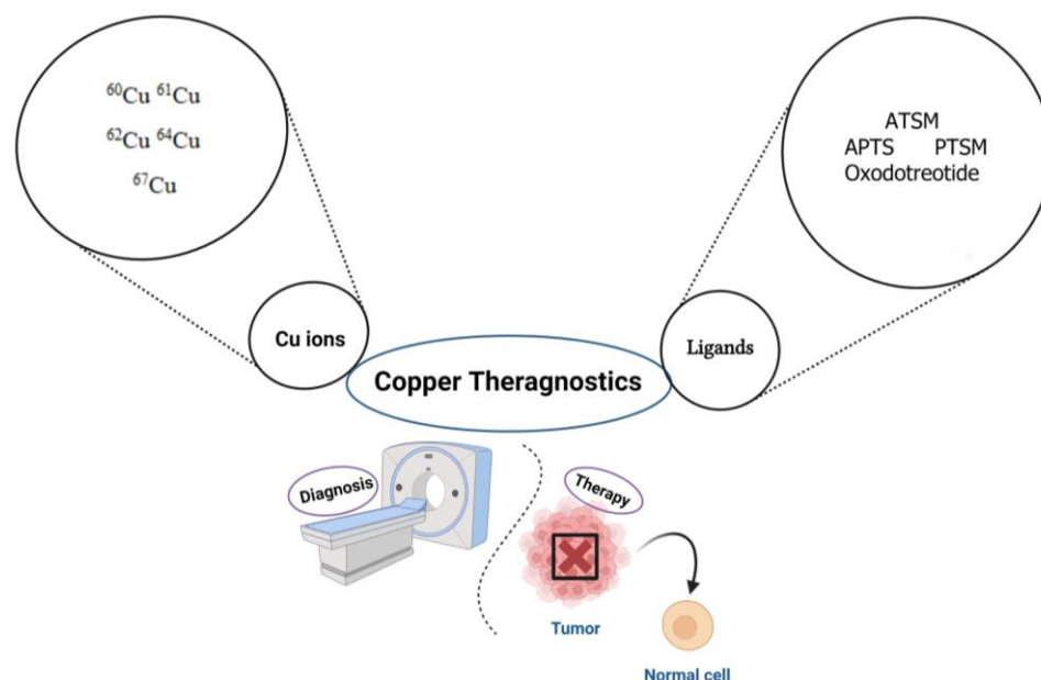
Figure 3. Major Cu ions and their ligands as promising theragnostic radionuclides for the diagnosis and treatment of different tumors. ^{60}\text{Cu} , ^{61}\text{Cu} , ^{62}\text{Cu} are labeled with ATSM, APTS, PTSM. ^{64}\text{Cu} is labeled with oxodotreotide (Dotatate). ^{67}\text{Cu} as a \beta^+ and \gamma -emitters can be used for both SPECT imaging and radiotherapy. ATSM: N4-methylthiosemicarbazone; APTS: 2-acetylpyridine thiosemicarbazone; PTSM: N4-methylthiosemicarbazone. Image created using Biorender ( https://www.biorender.com/ accessed on 22 August 2023).
