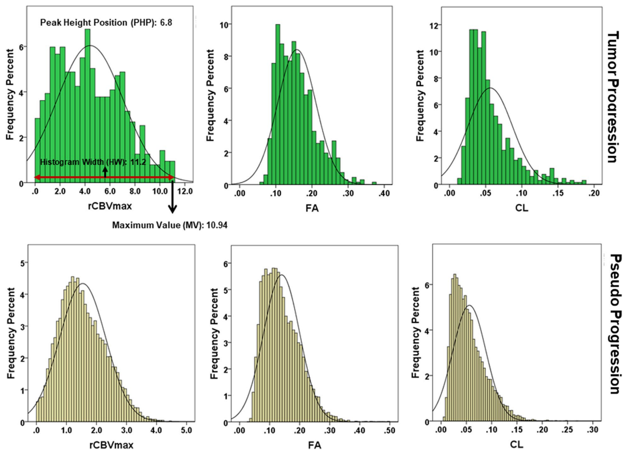
Fig. 4 Histograms showing the frequency distributions of parameters (FA, CL and rCBV) from entire volume of contrast-enhancing regions of neoplasms from two patients shown in Figs. 2 and 3. Please note the presence of greater peak height positions (PHP), histogram widths (HW) and maximum pixel values (MV) of these parameters in TP than in PsP
