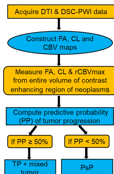
Fig. 1 The step-wise process of utilizing multiparametric MRI based prediction model in determining PsP and TP+mixed tumors
