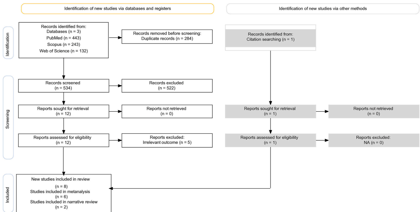
Fig. 1. Our current study's flowchart depicting that out of total of 818 articles, only six fulfilled our eligibility criteria and formed the basis of our meta-analysis.
