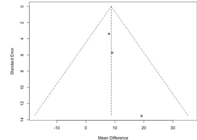
Fig. 9. Funnel plot of our paired meta-analysis. Due to the small number of the eligible studies, it was unclear to establish the presence of publication bias after eyeballing the funnel plot.
