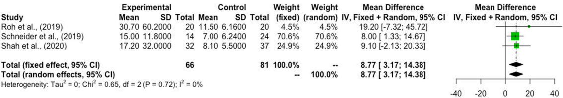
Fig. 8. A paired-meta-analysis was performed for comparing PFS between lobectomy and GTR. Mean difference in PFS between these approaches was 8.77 months (95% CI 3.17–14.38) in favor of lobectomy.
